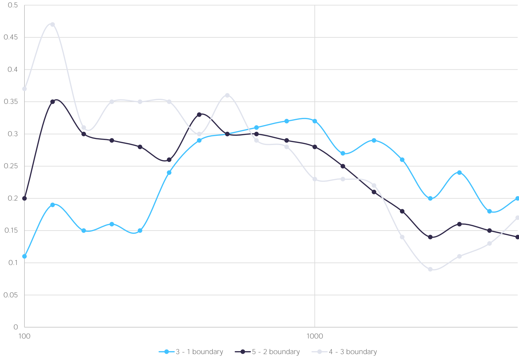
Equivalent Sound Absorption Per Object Areas - 3 Panels (1.08m 2 )
