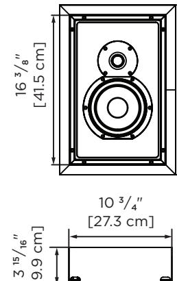
IN-WALL/4
